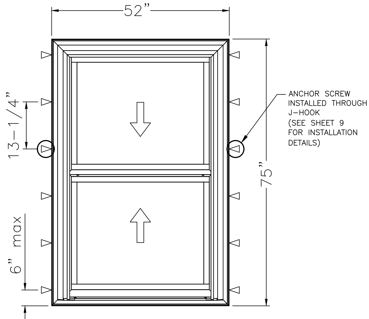
1650i PVC DH WINDOW – FINLESS INSTALLATION MAXIMUM SIZE 52" X 75" DESIGN PRESSURE +/- 50 PSF MISSILE D – WIND ZONE 3
