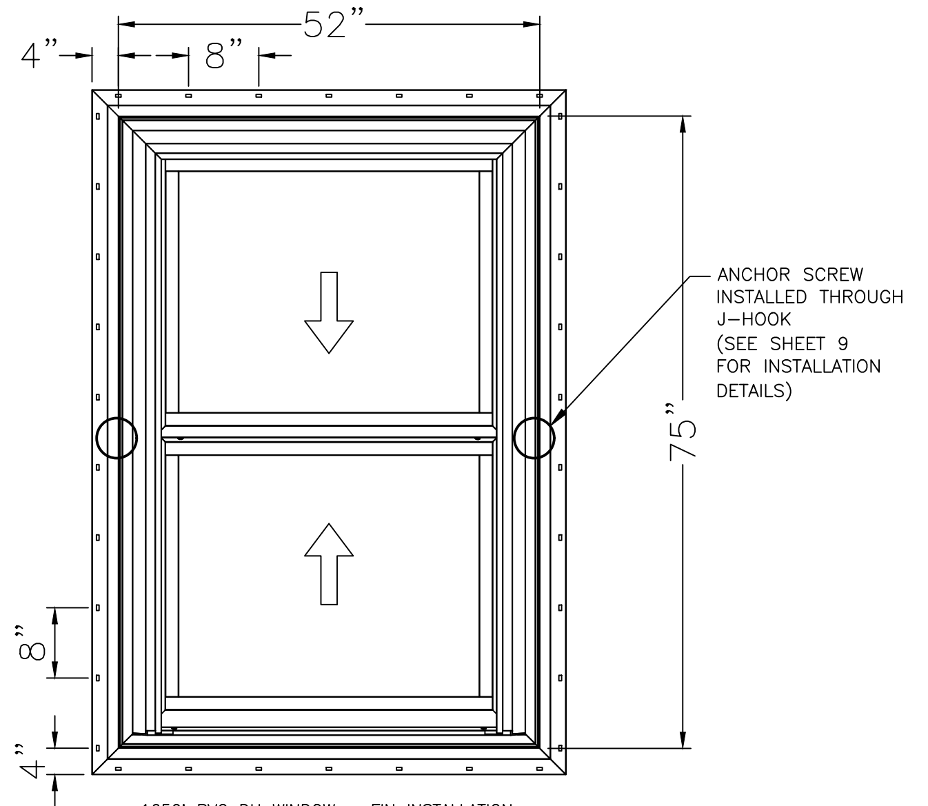
1650i PVC DH WINDOW – FIN INSTALLATION MAXIMUM SIZE 52" X 75" DESIGN PRESSURE +/- 50 PSF MISSILE D – WIND ZONE 3
